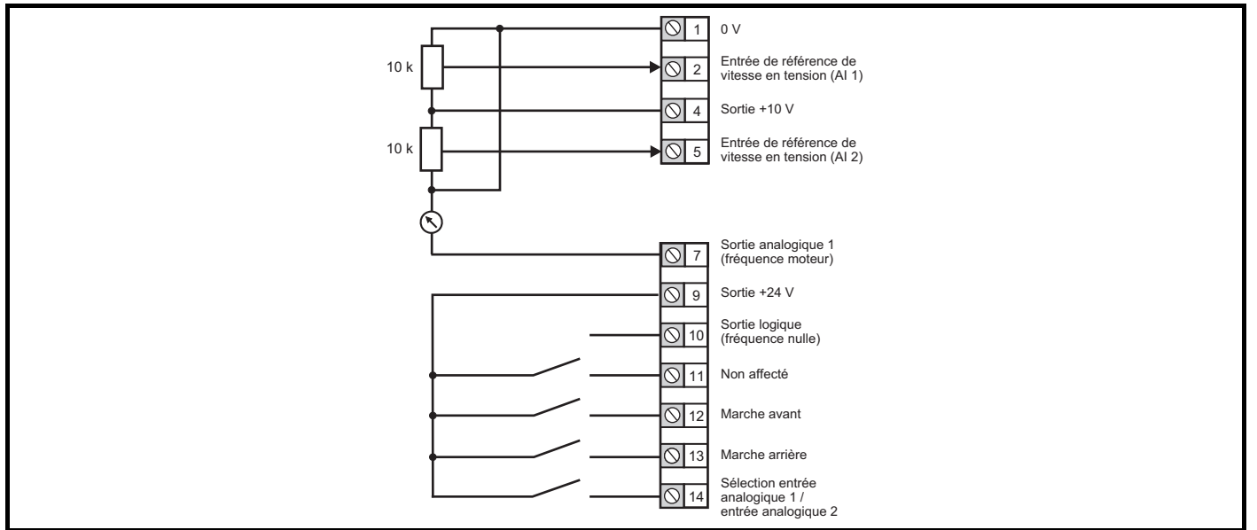
Figure 6-3 Pr 05 = AI
