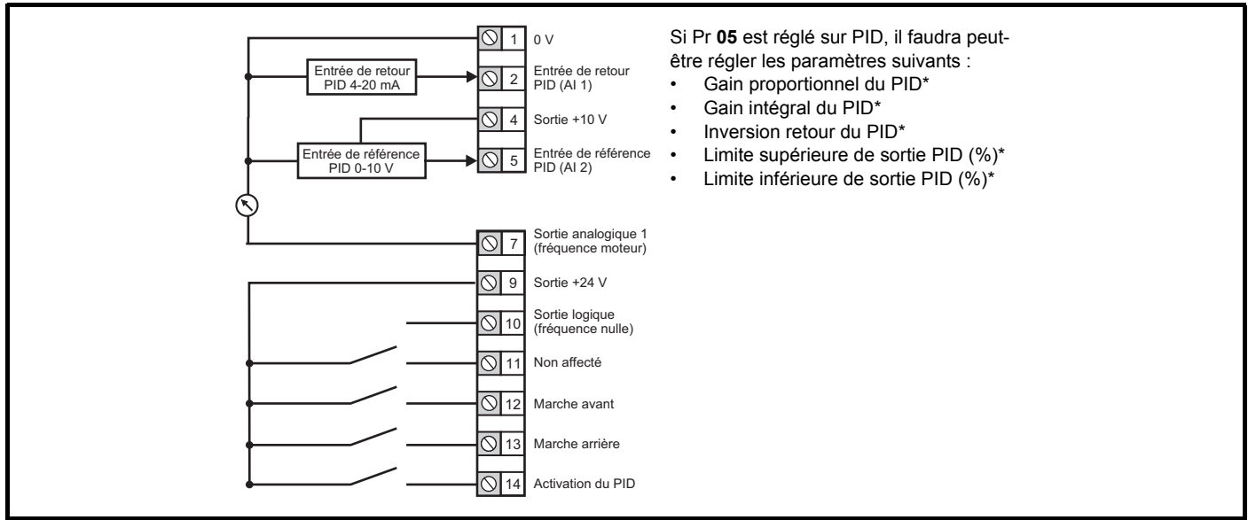
Figure 6-11 Pr 05 = Pid
