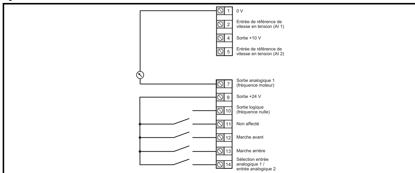
Figure 6-9 Pr 05 = E.Pot
