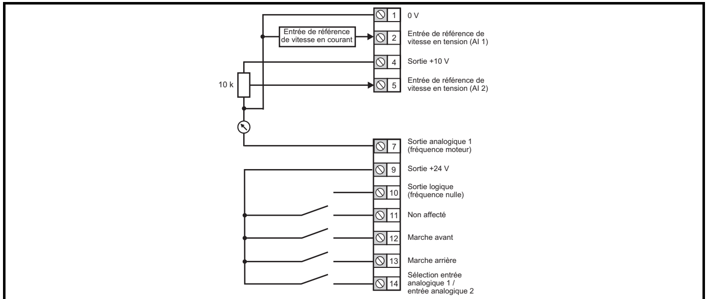
Figure 6-4 Pr 05 = AV.Pr
