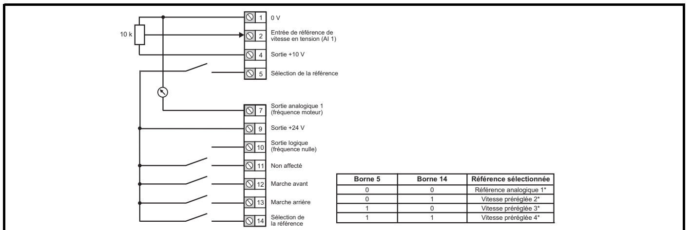
Figure 6-4 Pr 05 = AV.Pr
