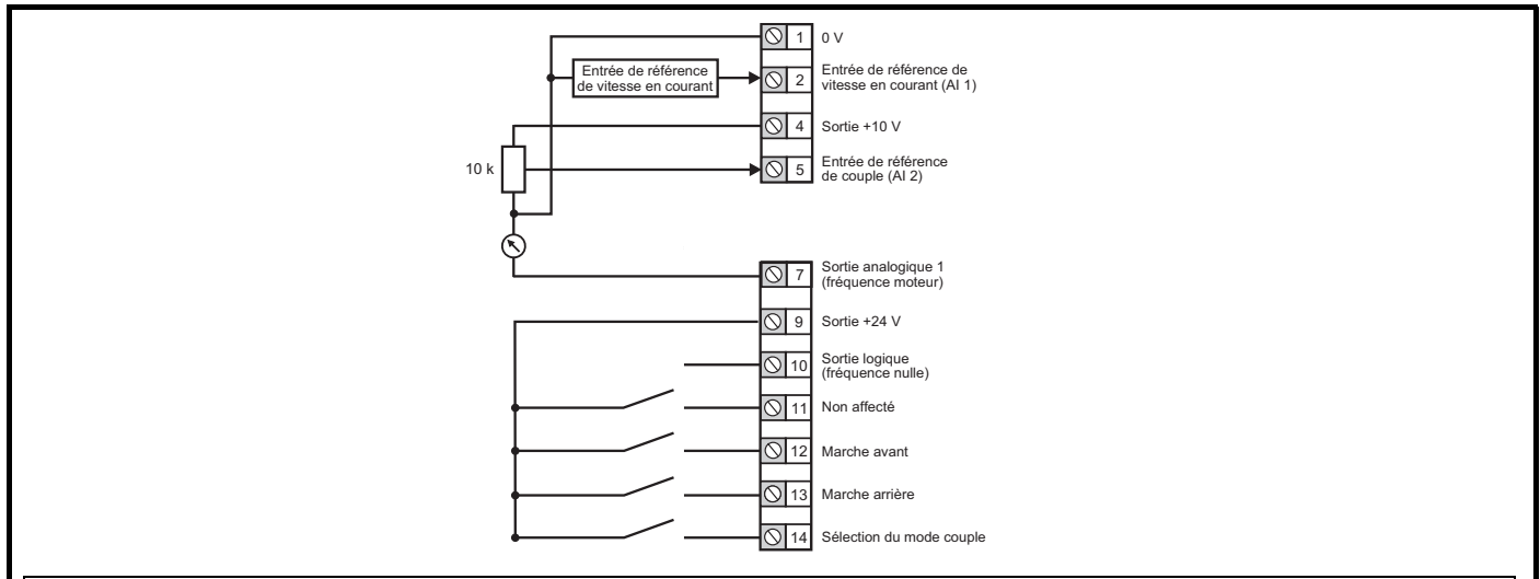
Figure 6-10 Pr 05 = torque
